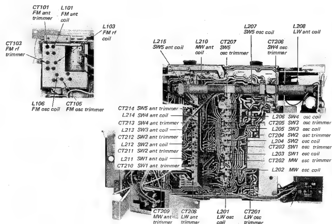
Fig. 3-10. Adjustment locations
